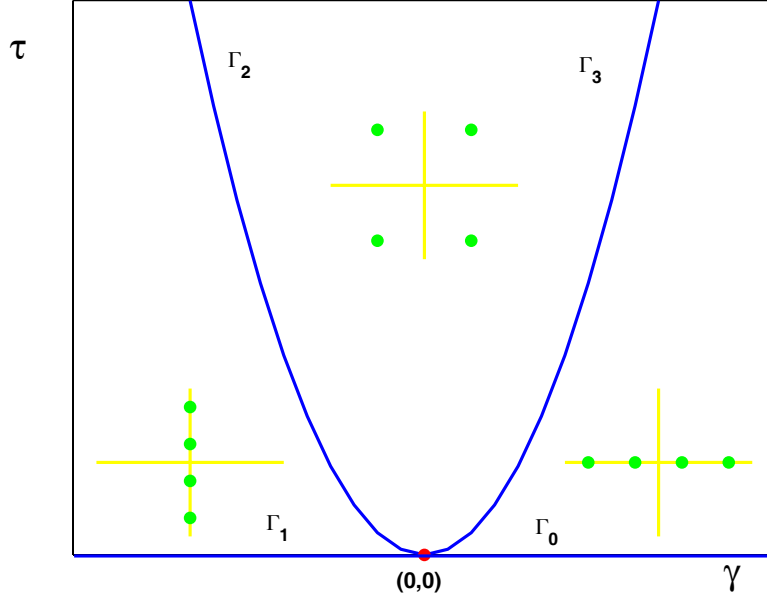
Figure 2: Eigenvalues of the scalar normal form (2.9) on the parameter plane (\gamma, \tau) . The curves \Gamma_{0,1,2,3} mark various bifurcations of co-dimension one.
