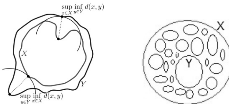
FIGURE 1. (left) Hausdorff distance between sets; (right) particular case where d_H(X, Y) does not capture the shape properties of X and Y .
