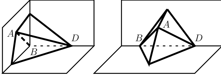
Figure 6: a B^2 -border and a B -border
