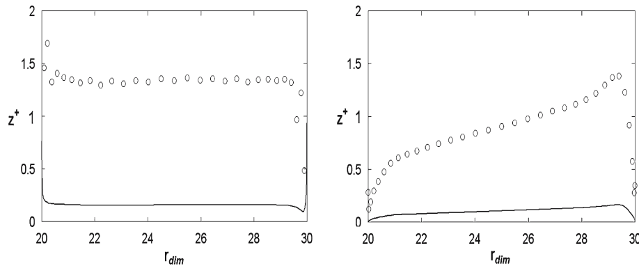
Fig. 5 Radial variation of the wall-normal value z^+ at the rotor ( left ) and at the stator ( right ) for Re = 7 \times 10^4 . Bold line DNS with grid 101 \times 200 \times 65 . Circles SVV-LES with grid 33 \times 64 \times 23
