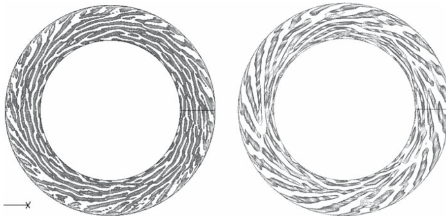
Fig. 6 Isolines of the velocity axial fluctuations in the stator boundary layer, Re = 7 \times 10^4 . DNS result with a 101 \times 200 \times 65 mesh ( left ) and SVV-LES result with a 33 \times 65 \times 23 mesh ( right )
