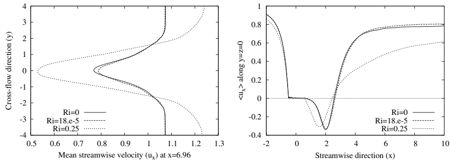
Fig. 2 For Ri = \{0, 18 \times 10^{-5}, 0.25\} , \langle u_x \rangle (y) at x \approx 7 (left) and \langle u_x \rangle (x) at y = 0 (right)
