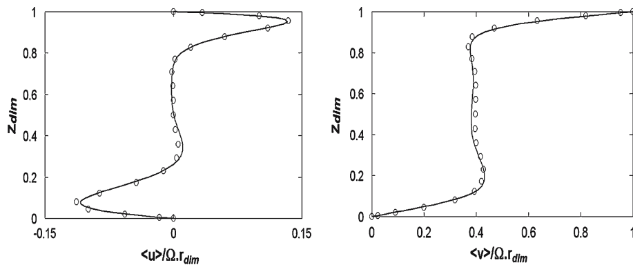
Fig. 7 Axial profiles of the radial (left) and tangential (right) components of the mean velocity at mid-radius, Re = 7 \times 10^4 . Bold line DNS with grid 101 \times 200 \times 65 . Circles SVV–LES with grid 33 \times 64 \times 23 . Results are normalized by the local velocity of the rotor \Omega r_{dim}
