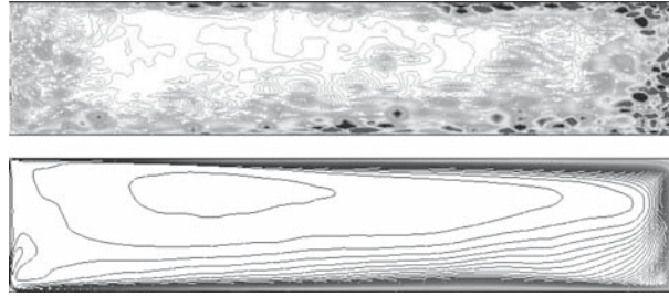
Fig. 9 Isolines of the instantaneous fields of Q -criterion for \theta = \pi/4 ( top ) and \theta -averaged turbulent kinetic energy ( bottom ), Re = 10^6
