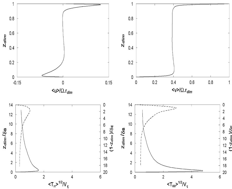
Fig. 10 Axial profiles at the mid radius of the mean radial velocity ( top left ), mean tangential velocity ( top right ), the square root of the radial ( bottom left ) and azimuthal ( bottom right ) normal Reynolds Stresses in the Ekman ( solid line ) and Bödewadt ( dashed line ) layers, Re = 10^6 . Mean velocities are normalized by the local velocity of the rotor. The square roots of the Reynolds stresses are normalized by the local friction velocity, V_\tau , on the corresponding disc
