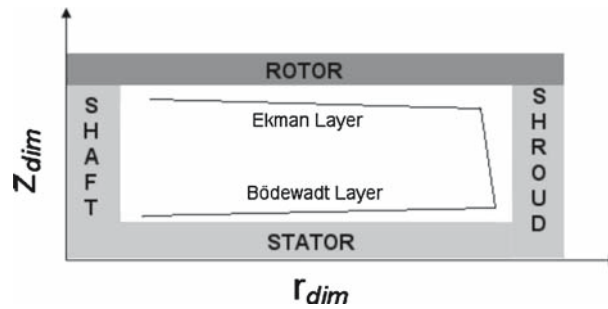
Fig. 4 Schematic of the rotor–stator cavity
