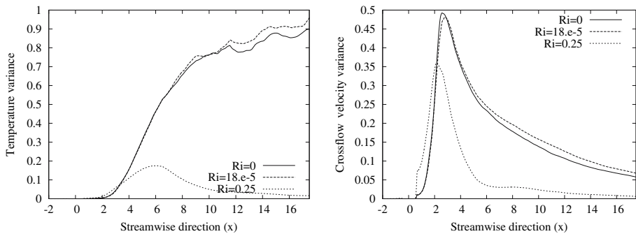
Fig. 3 For Ri = \{0, 18 \times 10^{-5}, 0.25\} , \langle T'^2 \rangle (x) (left) and \langle u_y'^2 \rangle (x) (right) at y = z = 0 (superscript prime represents deviation from the mean value)
