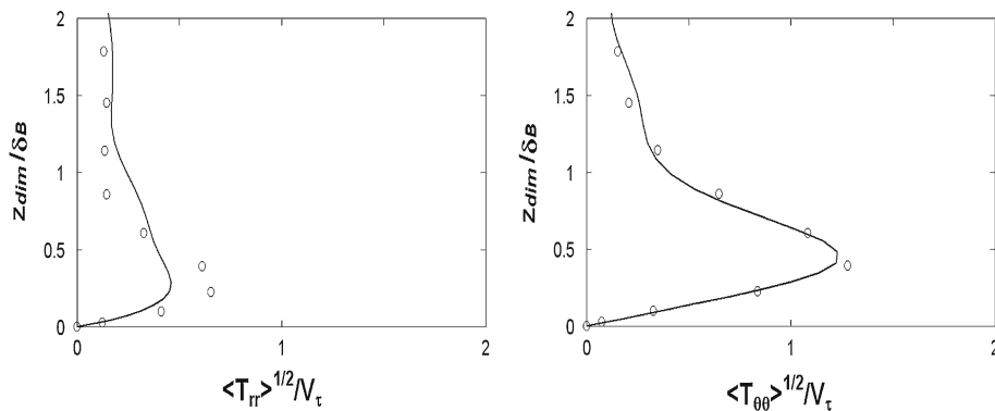
Fig. 8 Axial profiles of the radial (left) and tangential (right) normal Reynolds stresses in the stator boundary layer at the mid radius, Re = 7 \times 10^4 . Results are normalized by the wall friction velocity, V_\tau , on the stator. Bold line DNS with grid 101 \times 200 \times 65 . Circles SVV–LES with grid 33 \times 64 \times 23
