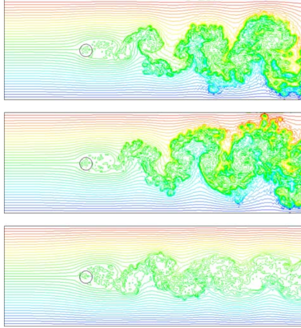
Fig. 1 Temperature field at z = 0 : Ri = 0 (top), Ri = 18 \times 10^{-5} (middle), and Ri = 0.25 (bottom)
